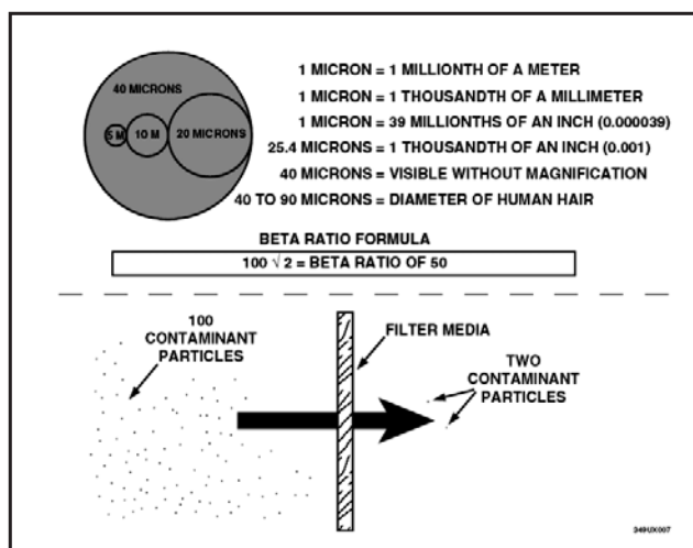
Micron Rating and Beta Ratio.
