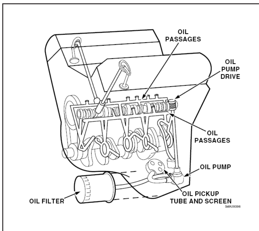
Typical engine lubrication system.
